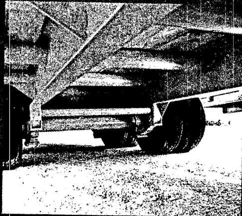
Mainframe — four I-beam construction with tubular crossmembers run through mainframe for lower deck height, greater strength and maximum deck rigidity against twisting.
